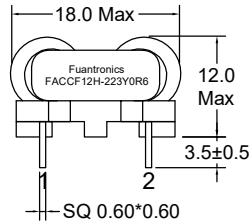
Orthographic view
